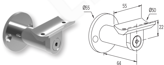
Supporto a muro per corrimano F50-200 Wall support for F50-200 handrail
