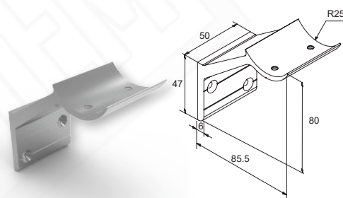
Supporto a parete per corrimano F50-200 Fixed wall support for F50-200 handrail
