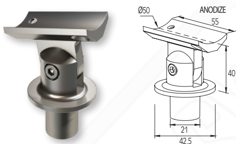
connettore per corrimano Ø50-colonna Ø42 (scala) Connector for handrail Ø50 with column Ø42 (stairs)
