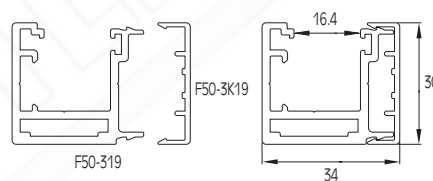
Cover per guida F50-319 Cover for guide F50-319
