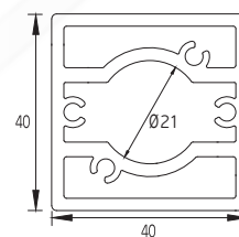
Colonna 40x40 Support column 40x40
