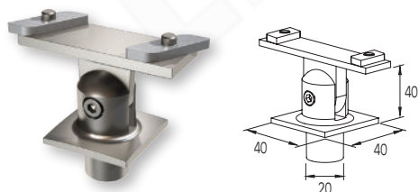
Connettore del corrimano F50-201 con colonna F50-102 Connector for F50-102 column with F50-201 handrail
