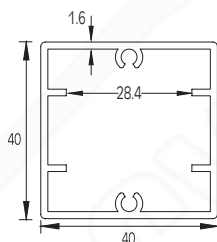
Colonna 40x40 Support column 40x40
