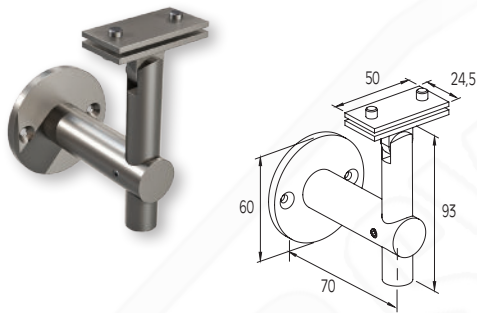
Supporto a parete F50-201 F50-201 Raitop wall support
