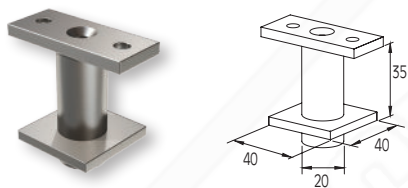
Connettore colonna F50-102 con corrimano F50-201 Support for F50-102 column with F50-201 handrail
