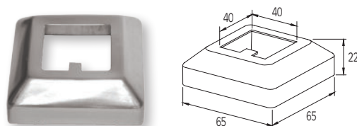
Cover a pavimento per colonna F50-102 Wall cover for F50-102 column
