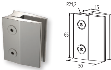
Supporto vetro 8-10 mm Glass support 8-10 mm
