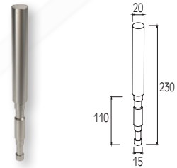
Supporto a pavimento per colonna F50-102 Infloor support for F50-102 column
