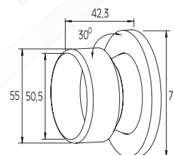
Cover a parete orientabile per corrimano Ø50 Wall cover for handrail Ø50 with cap
