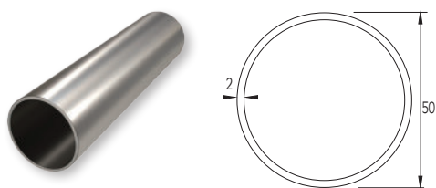
Corrimano Ø50 Handrail Ø50
