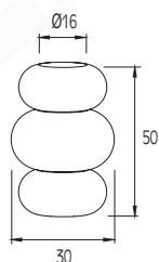
Borchia per profilo Ø16 Glass rosette for profile Ø16
